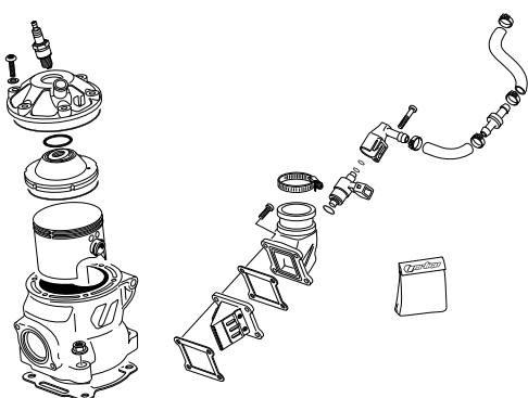
CILINDRO-CULATA-PISTON - CYLINDER-HEAD-PISTON
