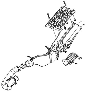
ESCAPE - EXHAUST
