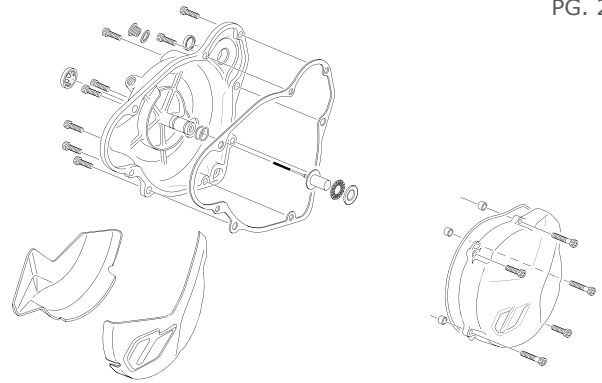
TAPAS - COVERS
