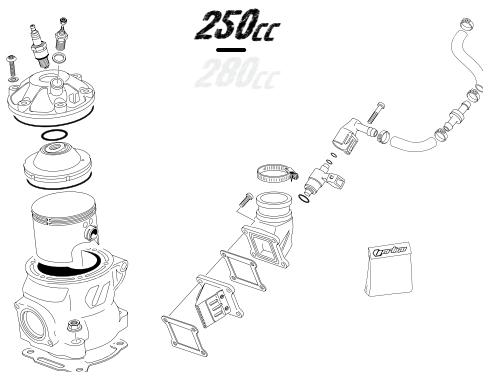
CILINDRO-CULATA-PISTON - CYLINDER-HEAD-PISTON
