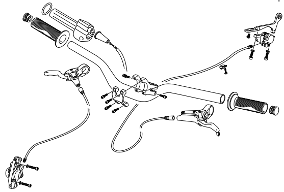
MANILLAR - HANDLEBAR
