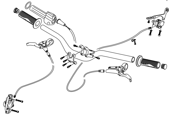
MANILLAR - HANDLEBAR
