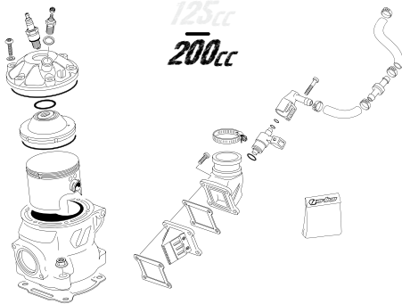
CILINDRO-CULATA-PISTON - CYLINDER-HEAD-PISTON
