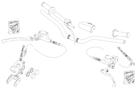
MANILLAR - HANDLEBAR
