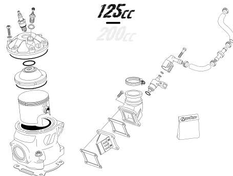
CILINDRO-CULATA-PISTON - CYLINDER-HEAD-PISTON
