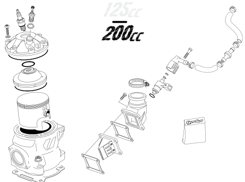
CILINDRO-CULATA-PISTON - CYLINDER-HEAD-PISTON
